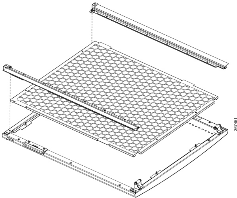
Figure 28: Align Door Filter to the Door
