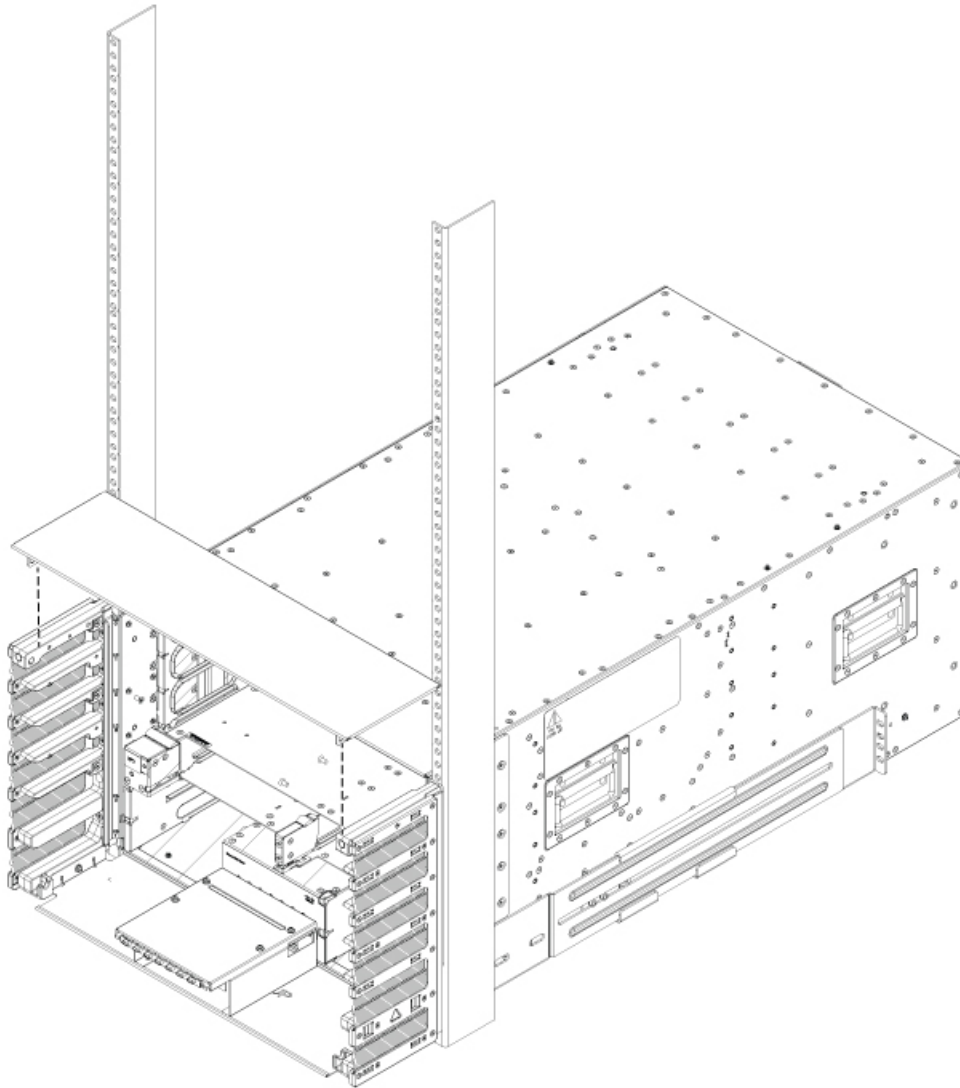
Figure 20: Attach Top Hood to NCS 5504 Chassis and Side Brush Filter Kit
