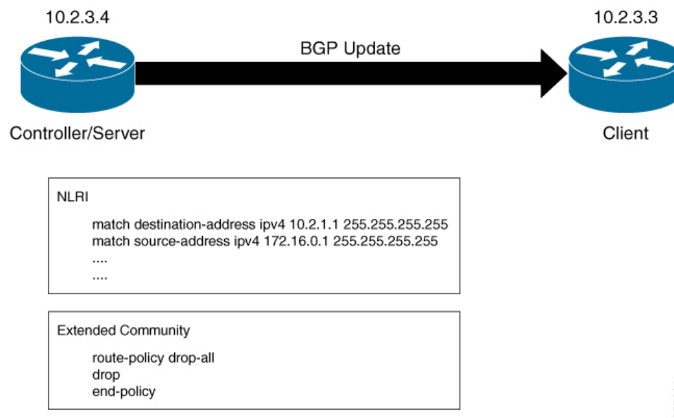
Figure 10: BGP Flowspec
