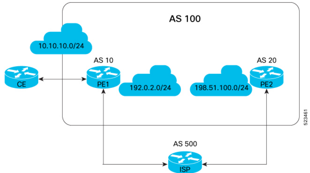
Figure 13: Topology
