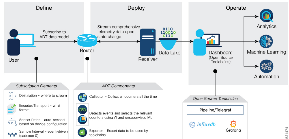
Figure 1: AI-Driven Telemetry
