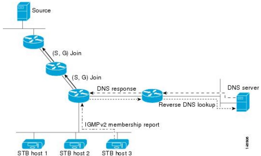
Figure 4: DNS-based SSM Mapping
