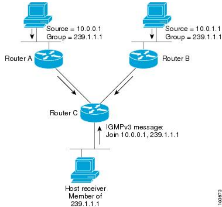
Figure 2: Designated Router Election on a Multiaccess Segment
