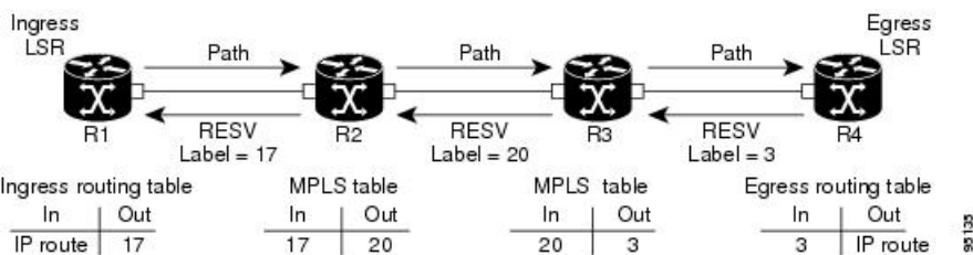
Figure 1: MPLS LSP Using RSVP
