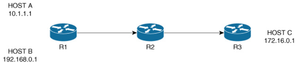
Figure 12: uRPF Topology
