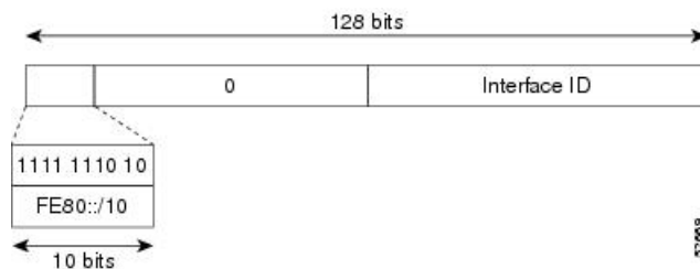
Figure 2: Link-Local Address Format
