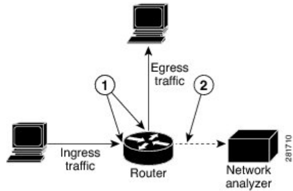
Figure 2: Network Analysis on a Cisco NCS 5000 Series Router With Traffic Mirroring
