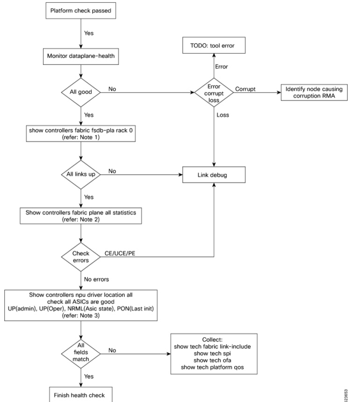
Figure 9: Troubleshooting Flowchart
