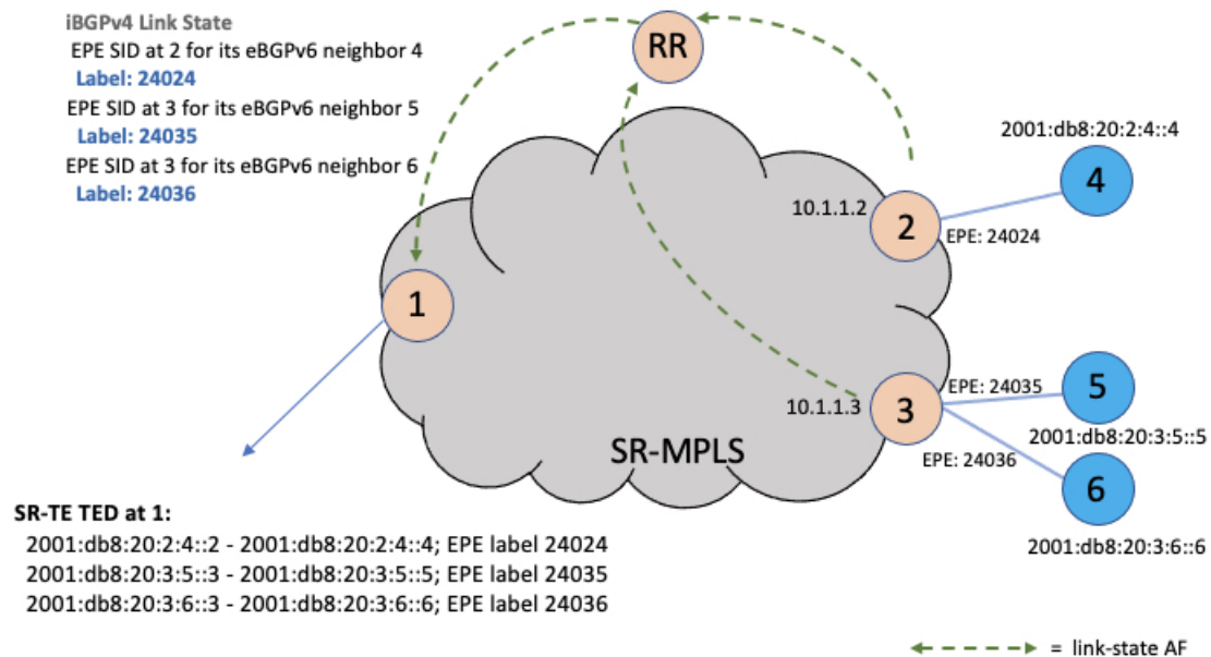
Figure 3: BGP-LS
