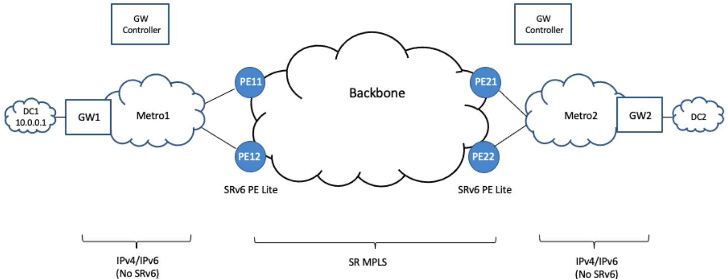
Figure 11: Example Topology
