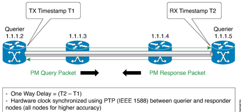
Figure 27: Performance Measurement for SR Policy End-to-End Delay
