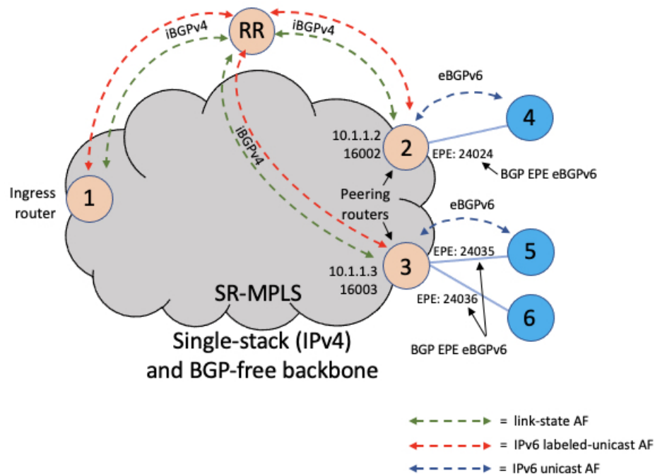
Figure 31: Network Setup
