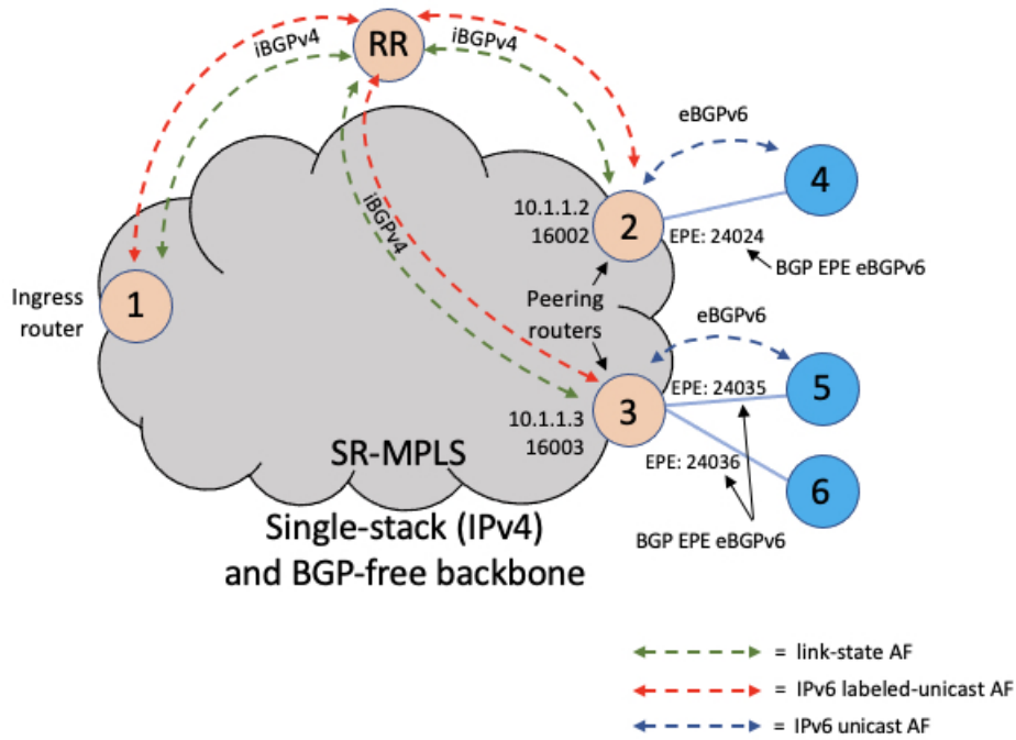
Figure 2: Network Setup
