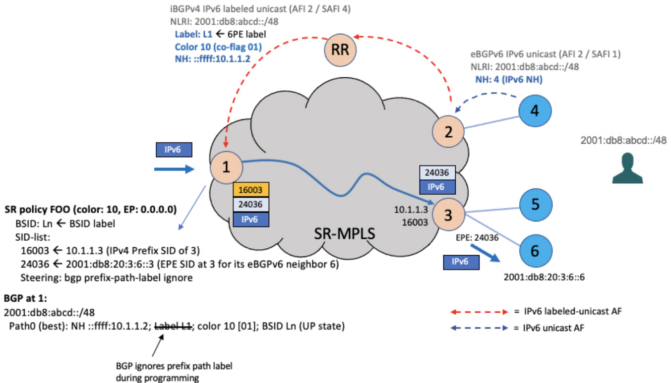
Figure 5: EPE Traffic-Engineered Path
