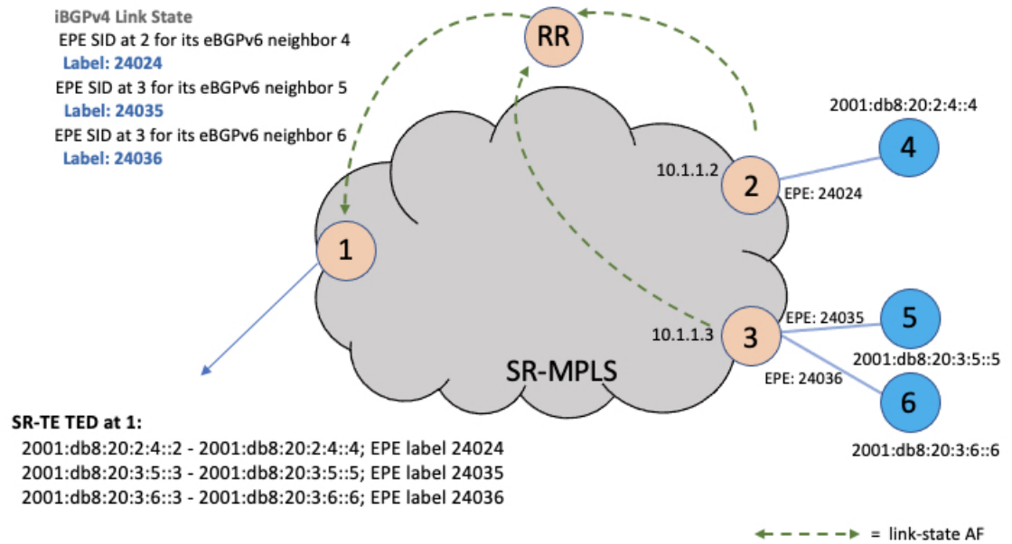
Figure 3: BGP-LS
