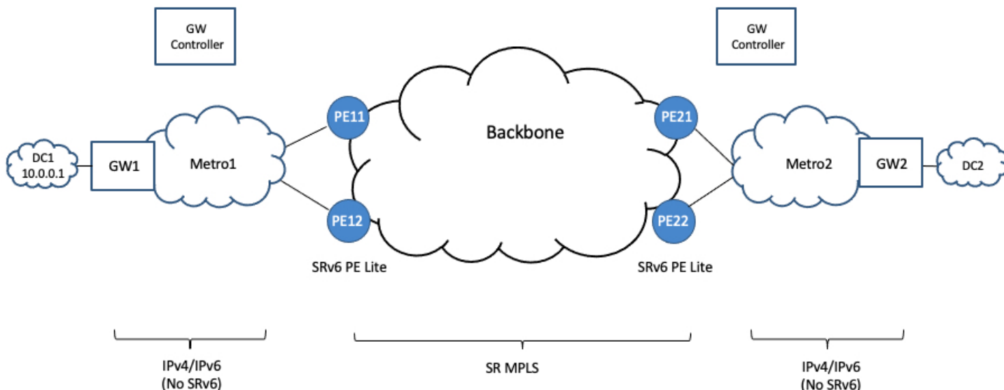
Figure 12: Example Topology
