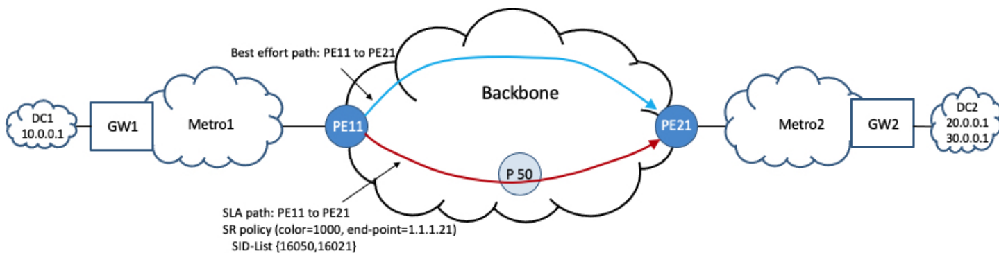
Figure 15: Backbone Transport Paths (Traffic Direction – DC1 to DC2)
