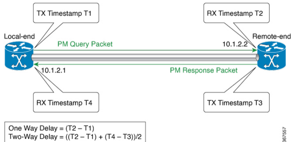
Figure 47: Performance Measurement for Link Delay
