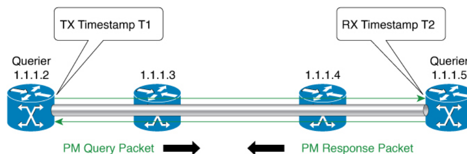
Figure 52: Performance Measurement for SR Policy End-to-End Delay
