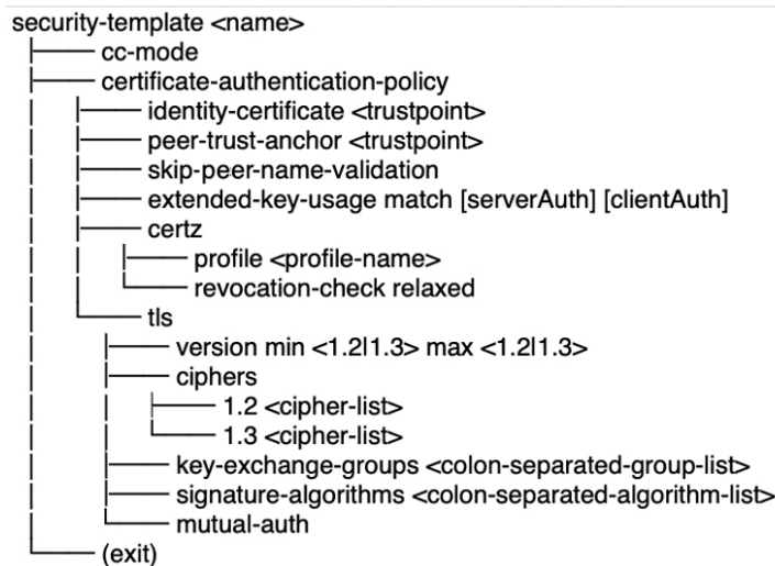
Figure 3: CLI Structure
