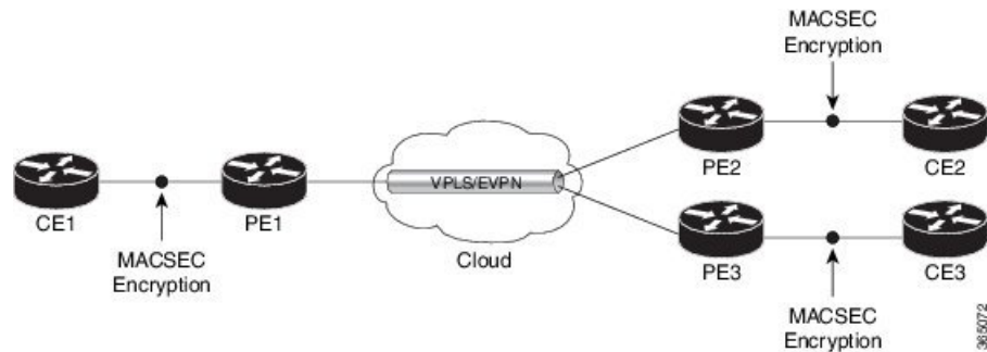
Figure 12: MACSec in a VPLS/EVPN Cloud
