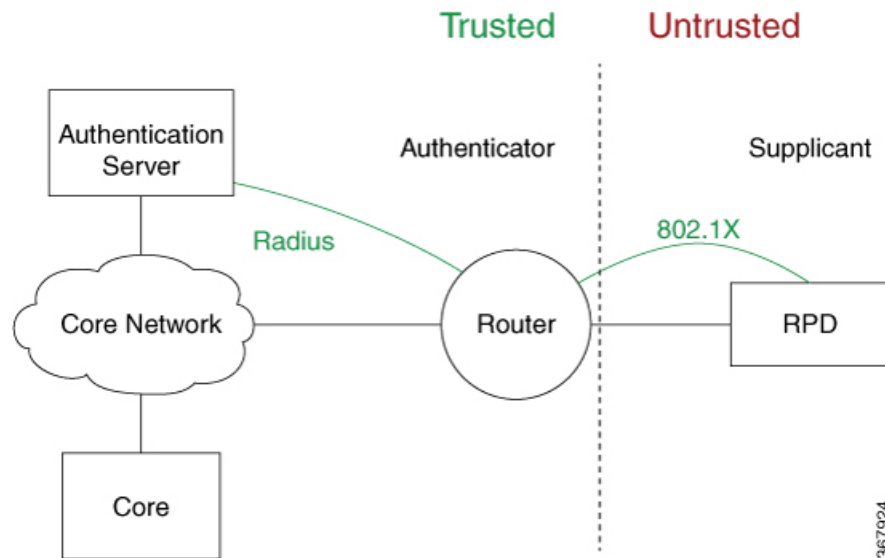
Figure 31: Topology for IEEE 802.1X Port-Based Authentication
