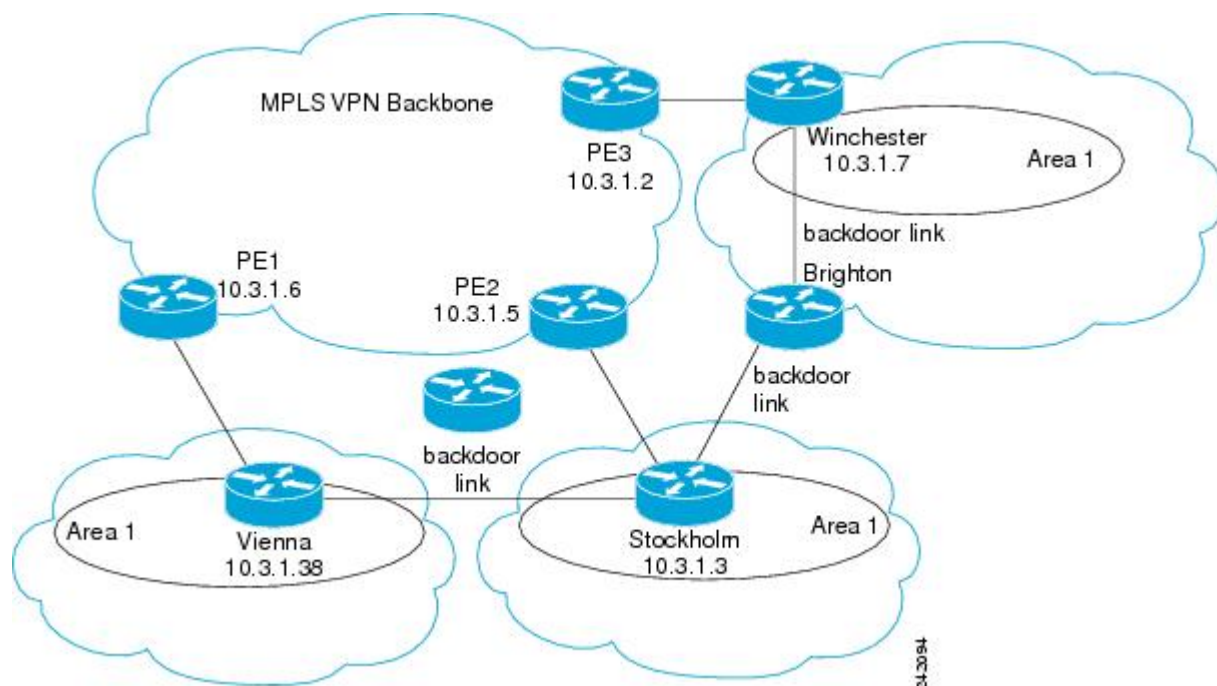
Figure 3: Backdoor Paths Between OSPF Client Sites
