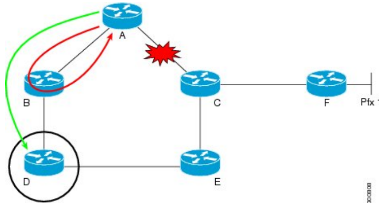
Figure 1: FRR with Remote LFA with Ring Topology
