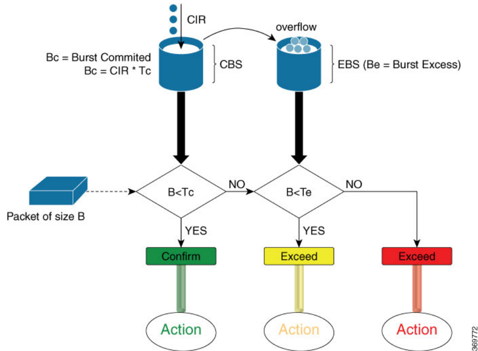
Figure 11: Workflow of Single-Rate Two-Color Policing
