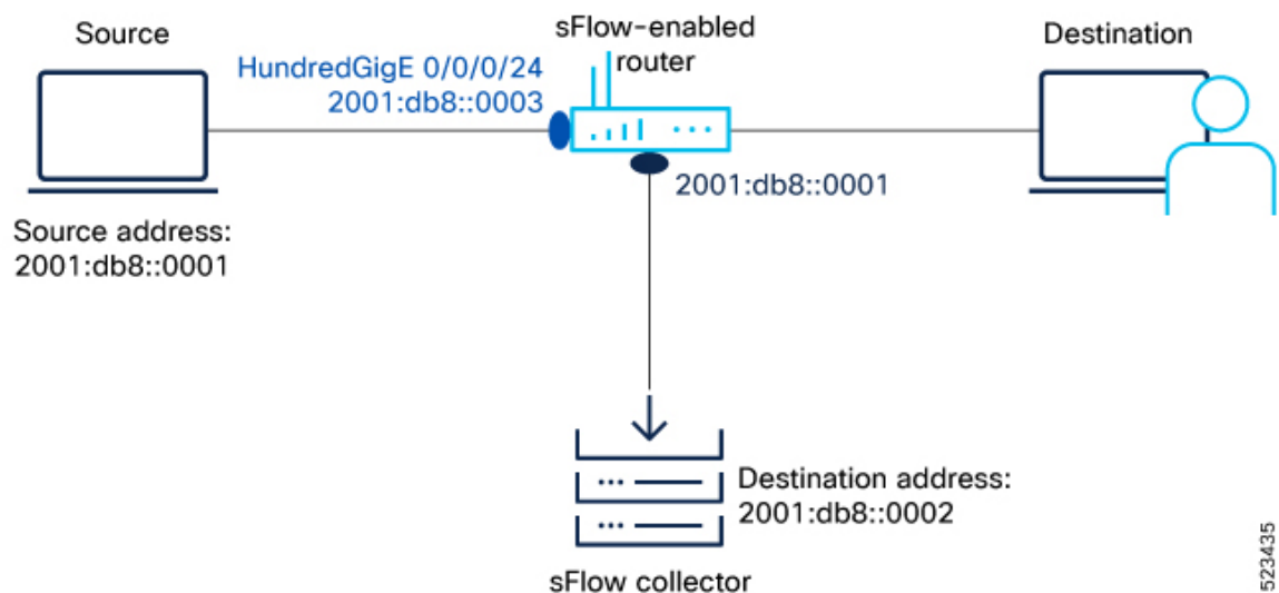
Figure 2: sFlow Configuration
