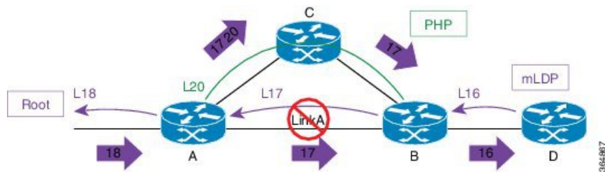
Figure 7: Link Failure
