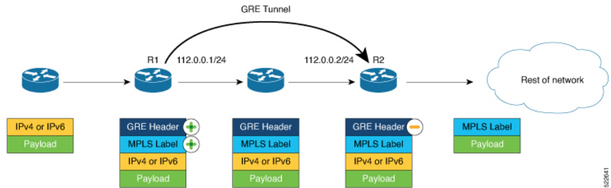
Figure 12: MPLS Over GRE Tunnel
