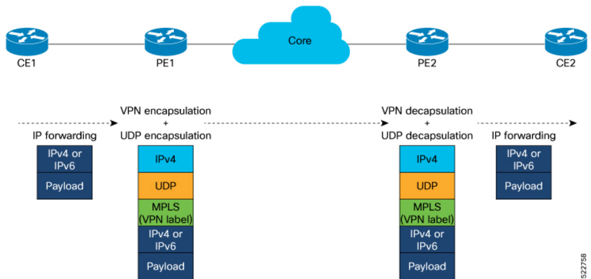
Figure 14: MPLS over UDP
