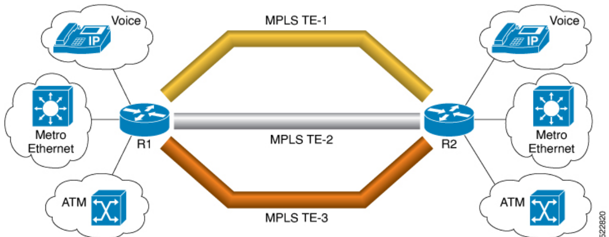
Figure 15: Policy-Based Tunnel Selection
