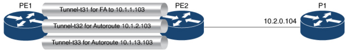
Figure 3: Topology
