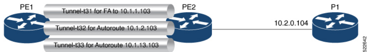
Figure 2: Topology
