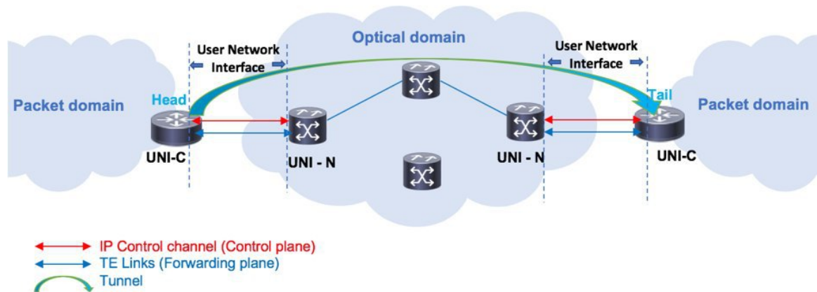
Figure 25: GMPLS UNI
