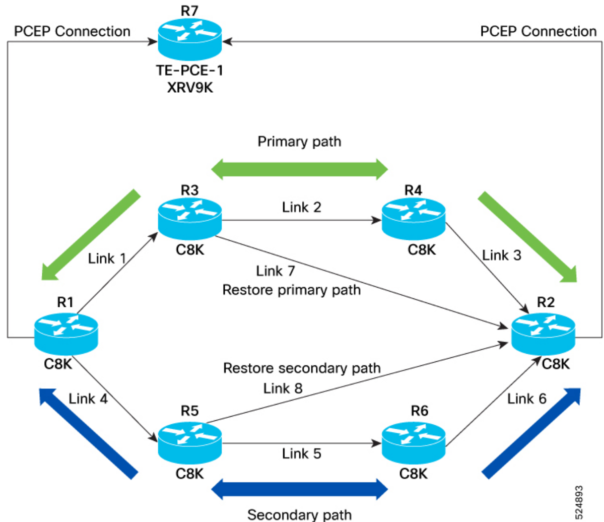
Figure 23: Flex LSP path computation using PCE
