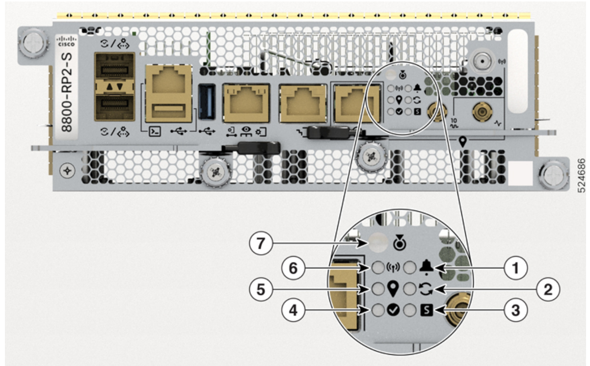
Figure 6: Route Processor LEDs - 8800-RP2-S
