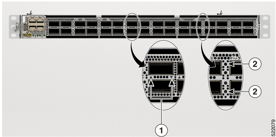
Figure 15: Port Status LED - Cisco 8201-32FH Chassis
