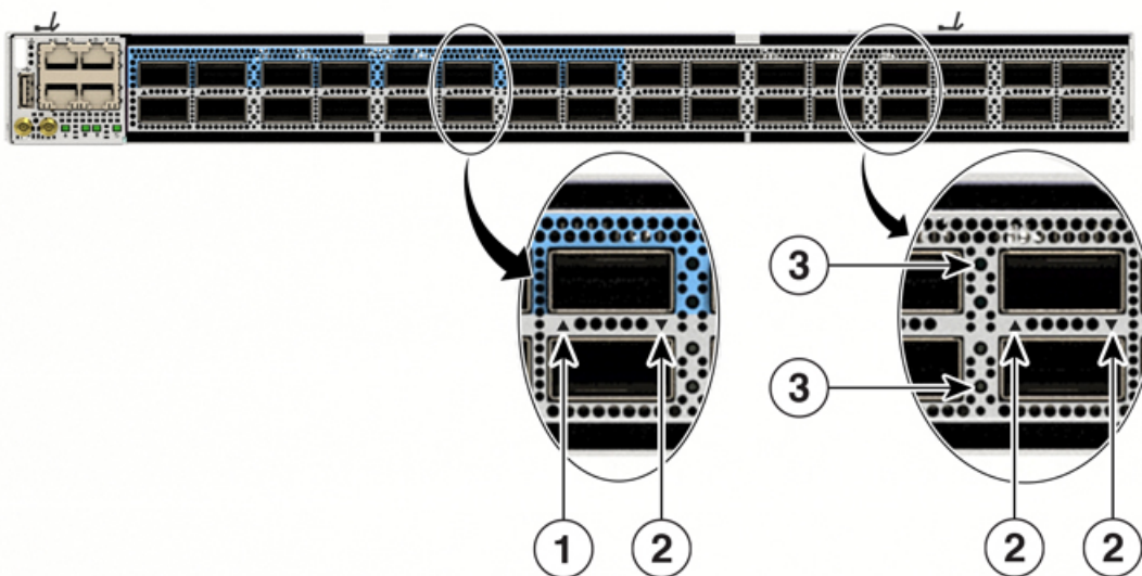
Figure 17: Port Status LED - Cisco 8201-24H8FH Router
