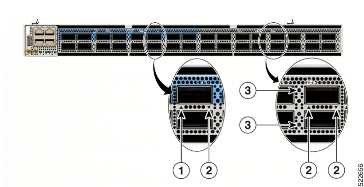
Figure 20: Port Status LED - Cisco 8201-24H8FH Router
