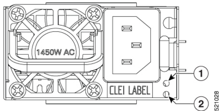
Figure 10: Power Supply LED - 1450W
