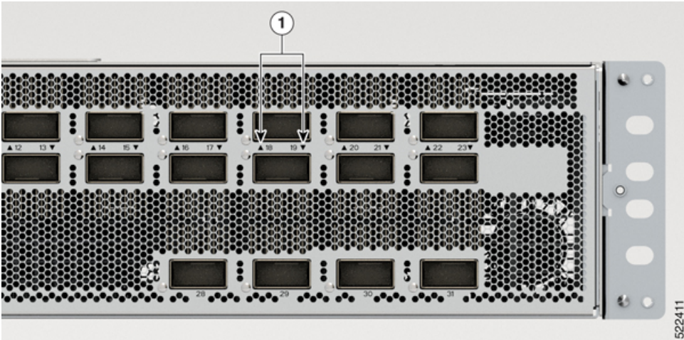
Figure 18: Port Status LED - Cisco 8202-32FH -M Chassis
