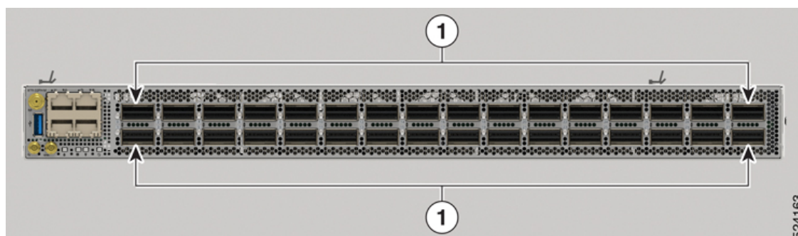
Figure 1: Cisco 8711-32FH-M - Front View
