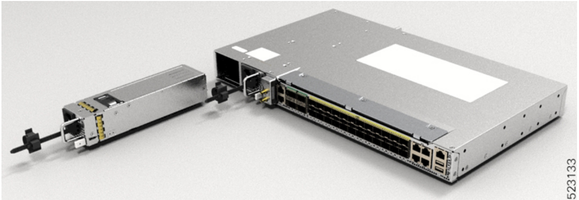
Figure 2: Install AC Power Supply Module
