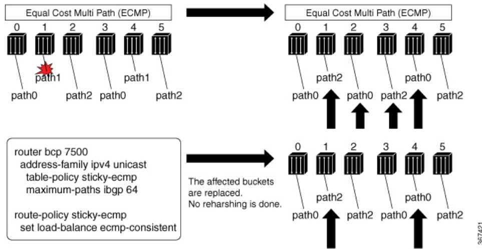
Figure 12: Resilient hashing and flow auto-recovery
