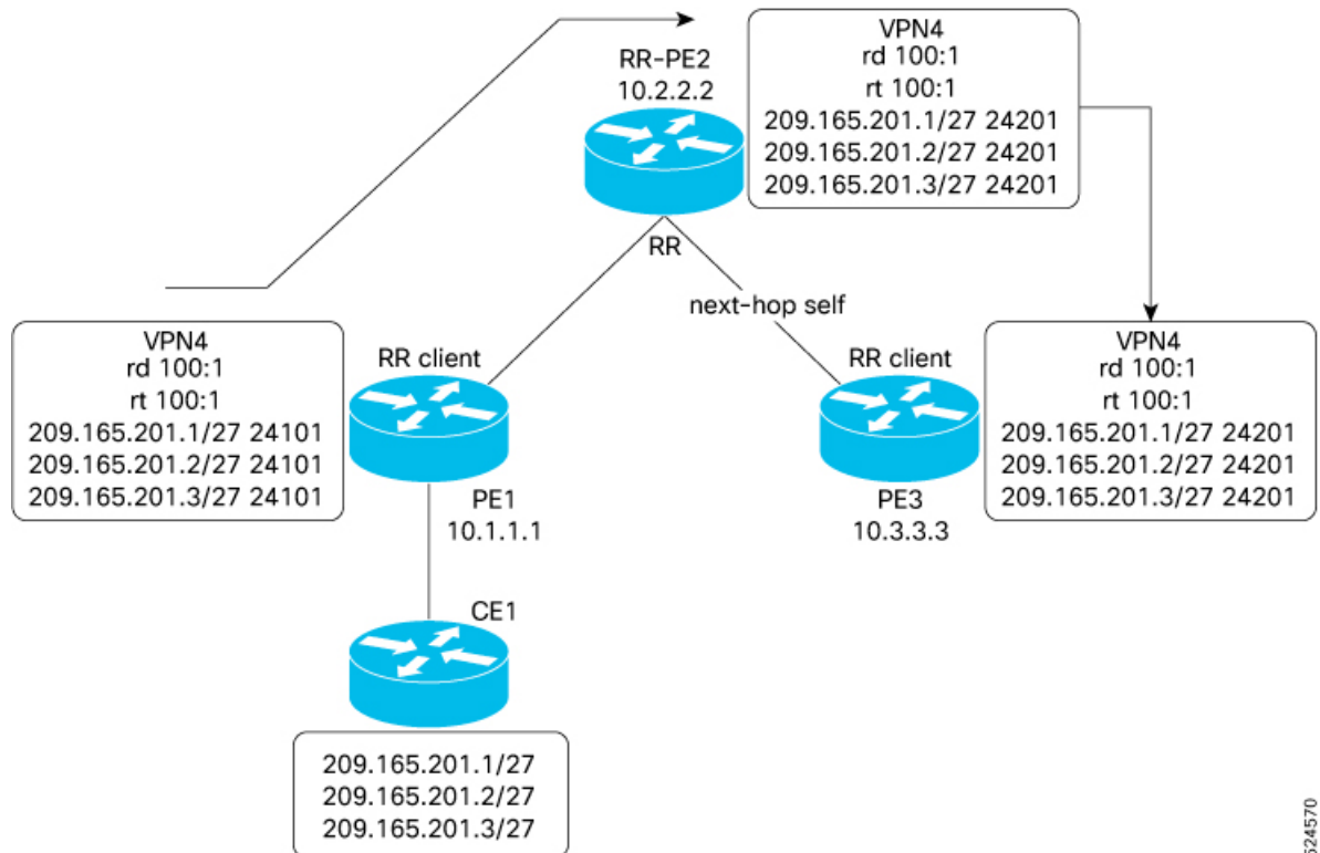
Figure 23: Sample topology for same RD configuration
