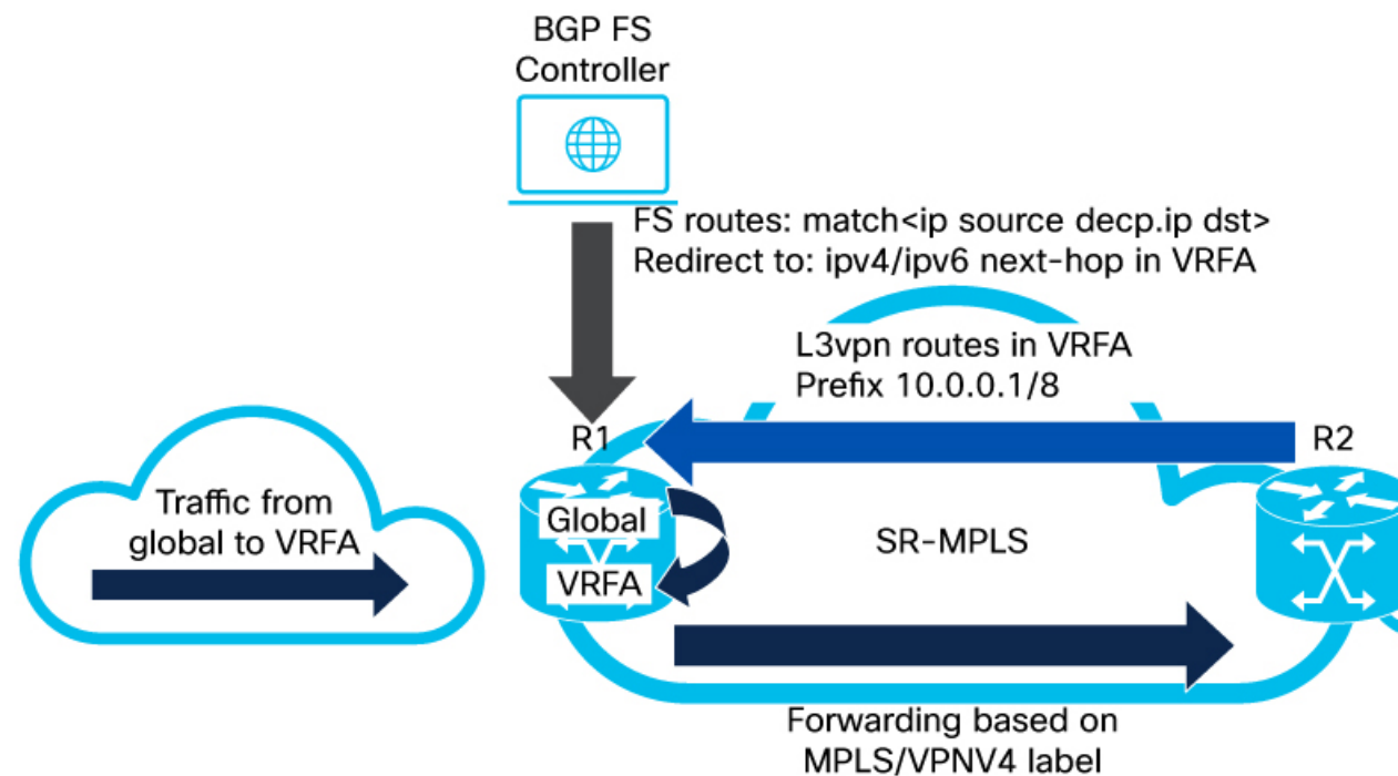
Figure 28: Forwarding based on MPLS
