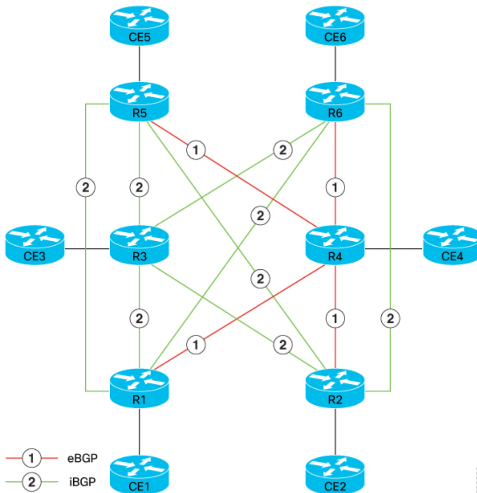
Figure 10: Example topology
