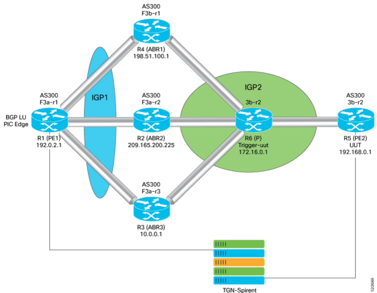
Figure 22: BGP labeled unicast prefix independent convergence edge
