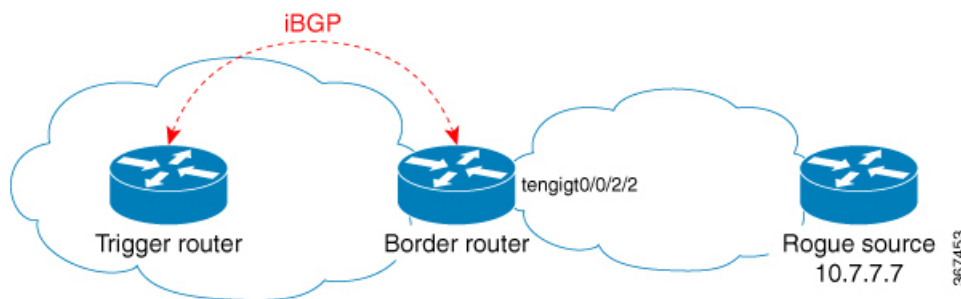
Figure 17: Topology to implement RTBH filtering
