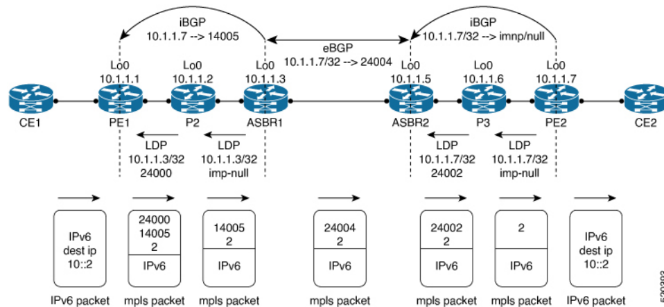
Figure 20: 6PE over BGP LU (inter-AS option C) control plane and data plane
