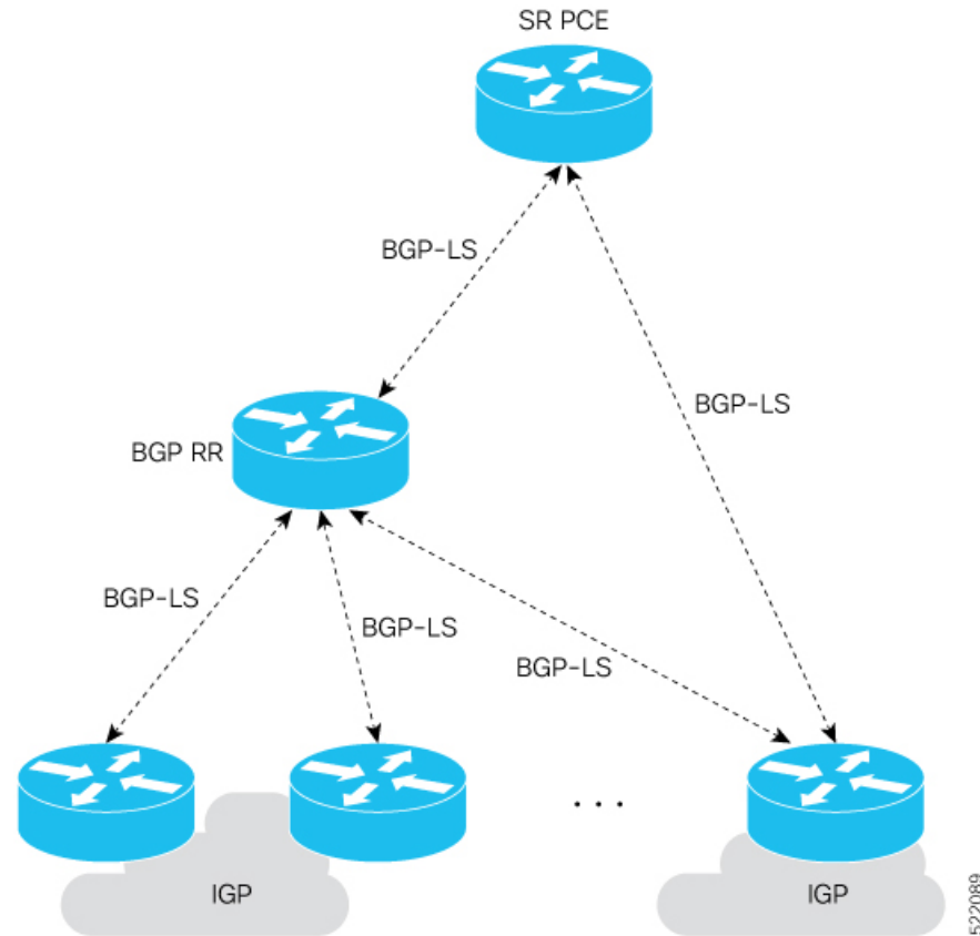
Figure 7: Deployment scenario for BGP-LS
