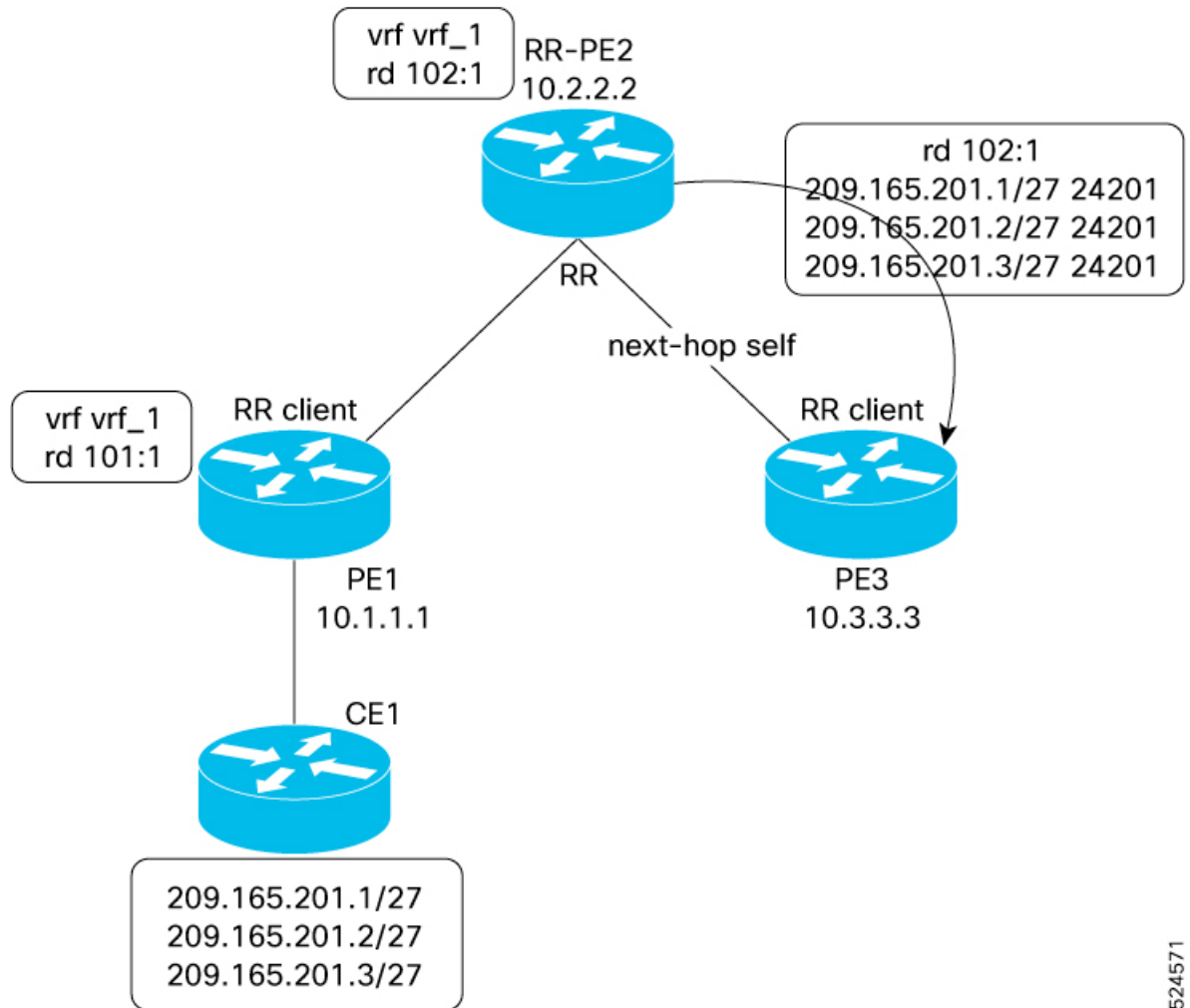
Figure 24: Sample topology for different RD configuration
