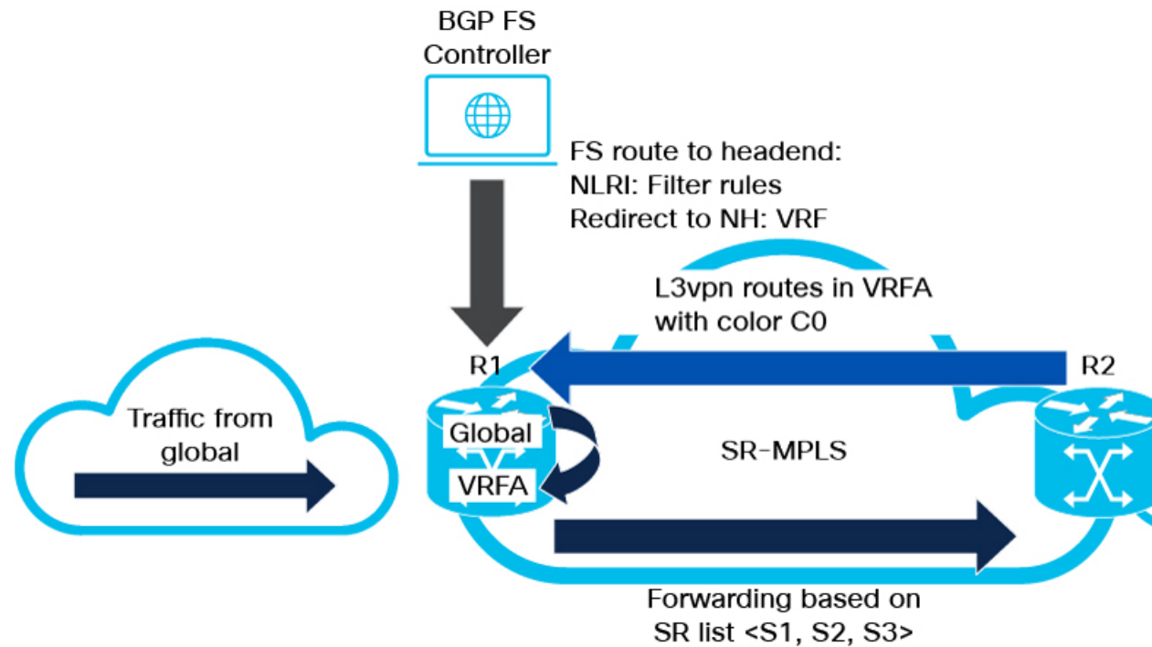
Figure 28: Forwarding based on MPLS
