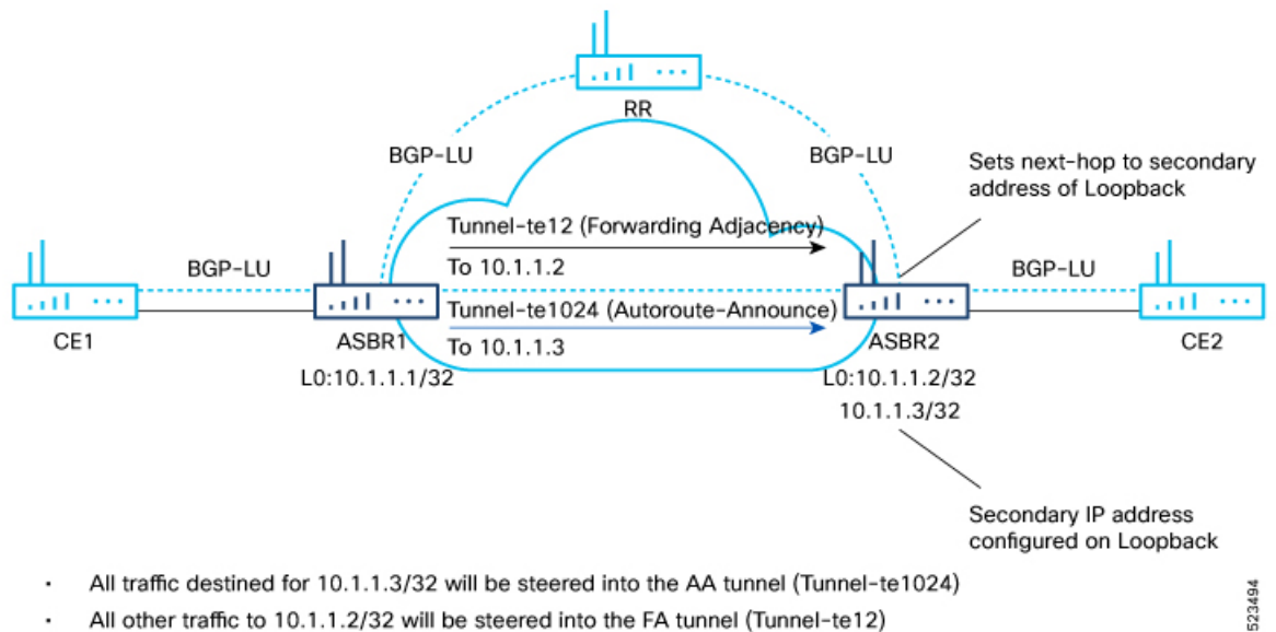
Figure 21: BGP labeled unicast over RSVP-TE
