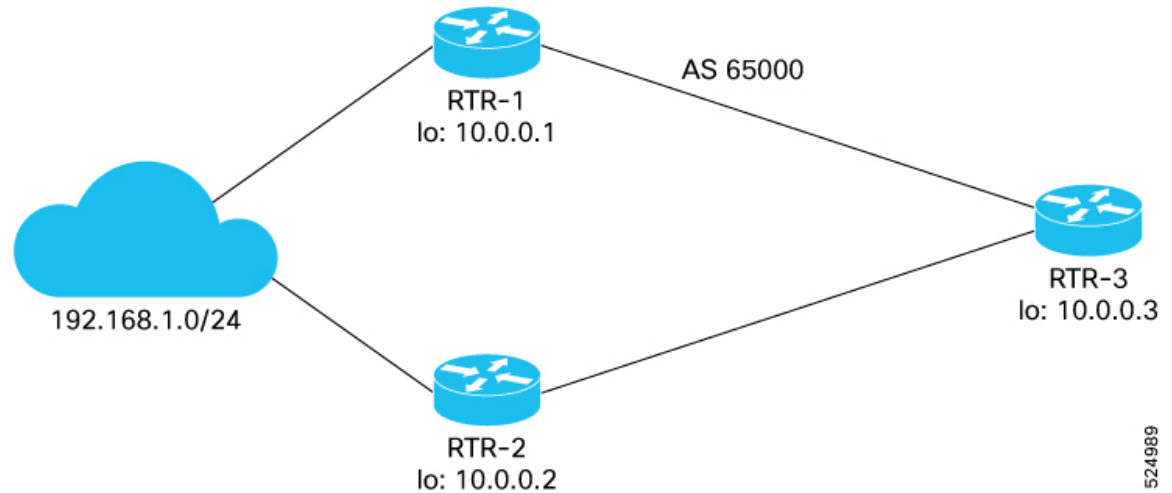
Figure 16: Example topology for bandwidth-aware BGP path selection using UCMP
