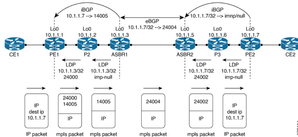
Figure 19: BGP labeled unicast (Intra-Autonomous System Option C) control plane and data plane
