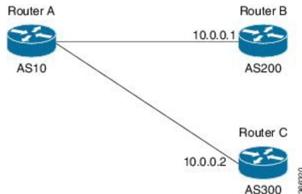
Figure 9: Connection topology with dynamic neighbors from multiple remote ASes
