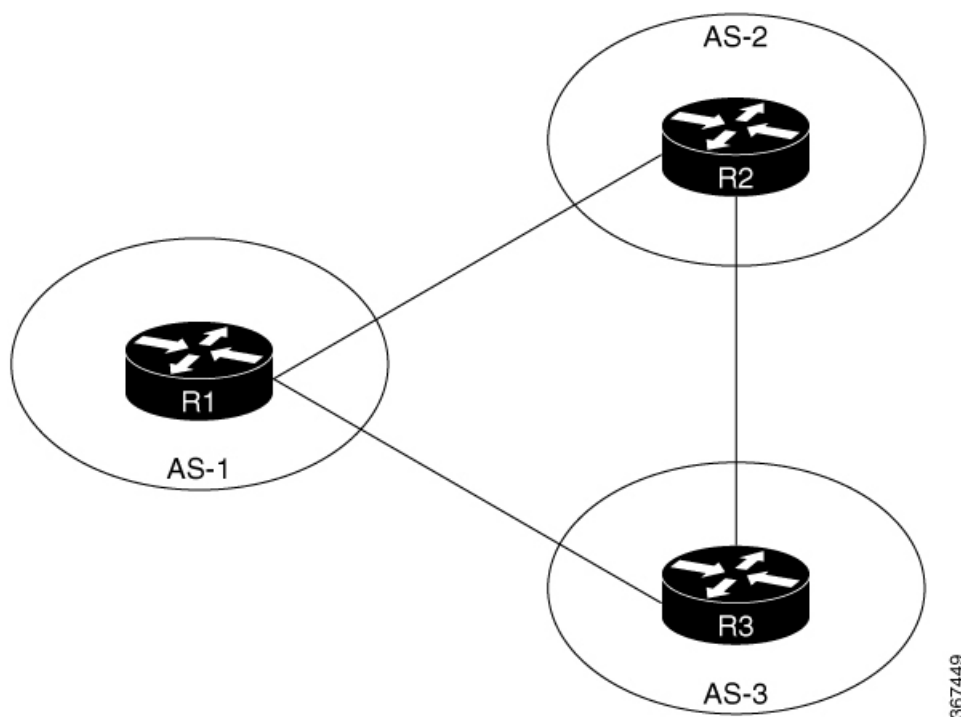
Figure 14: Topology example: routing loop formation
