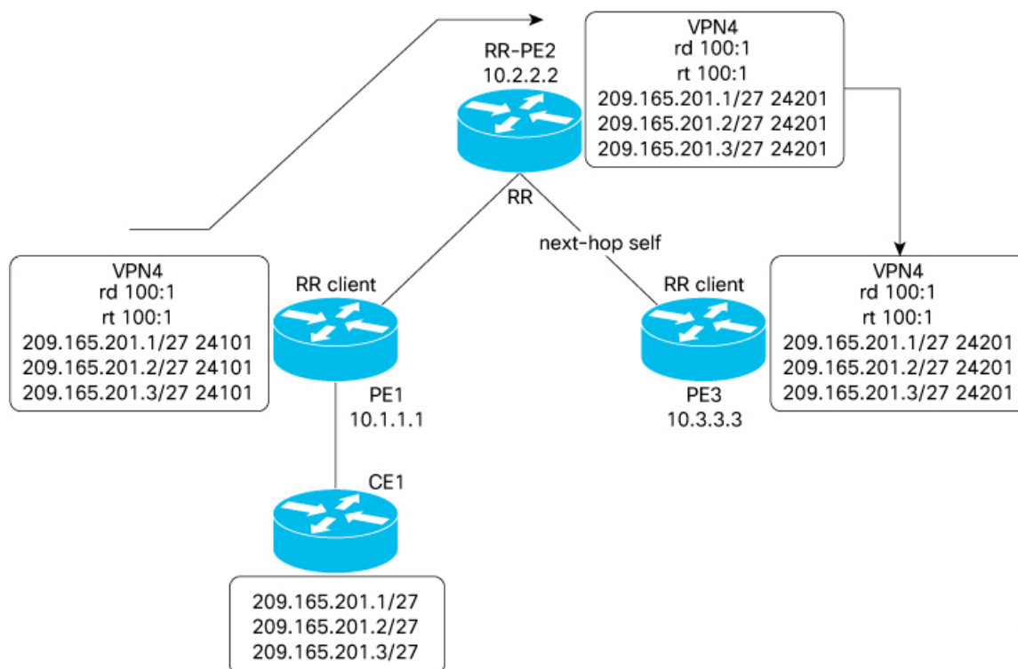
Figure 22: Sample topology for same RD configuration
