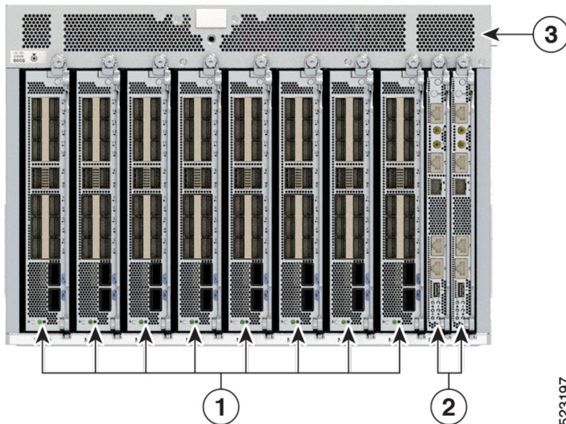
Figure 18: Redundant Set of RP Installed in Slots RP0 and RP1 in an Cisco 8608 8-Slot Centralized Chassis
