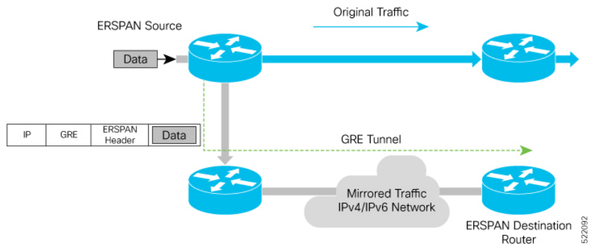
Figure 12: ERSPAN over GRE
