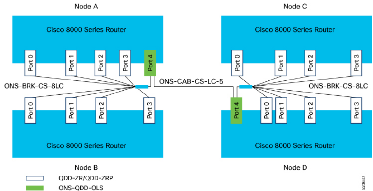
Figure 25: 8-Channel Optical Line System
