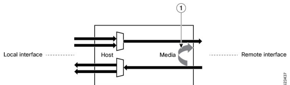
Figure 19: Media Side Input Loopback on the Optical Transceiver
