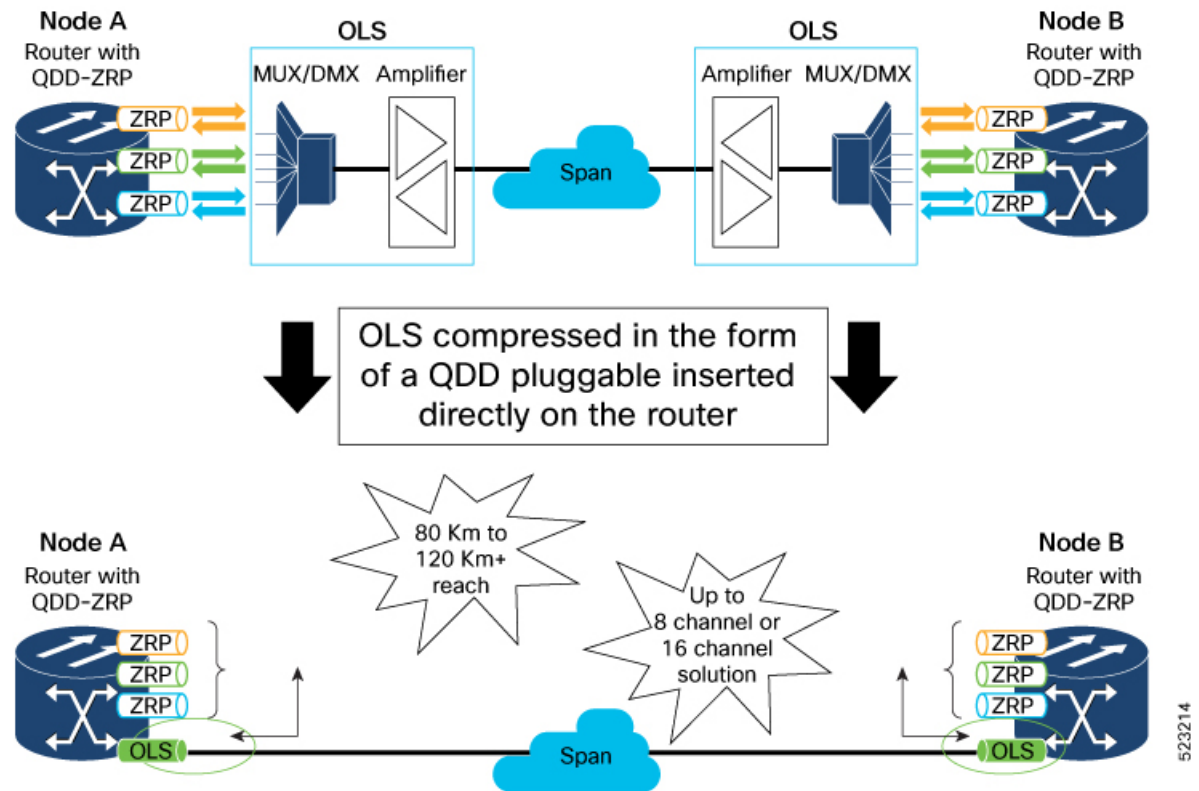
Figure 23: QDD Optical Line System
