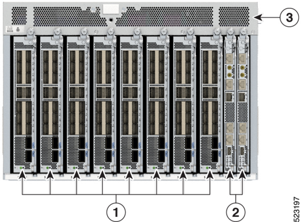
Figure 26: Redundant Set of RP Installed in Slots RP0 and RP1 in an Cisco 8608 8-Slot Centralized Chassis
