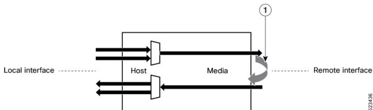
Figure 20: Media Side Output Loopback on the Optical Transceiver
