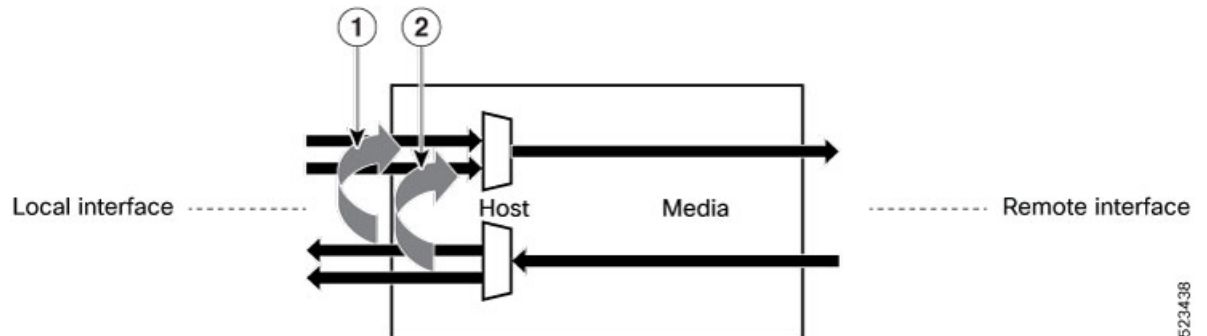
Figure 4: Host Side Output Loopback on the Optical Transceiver
