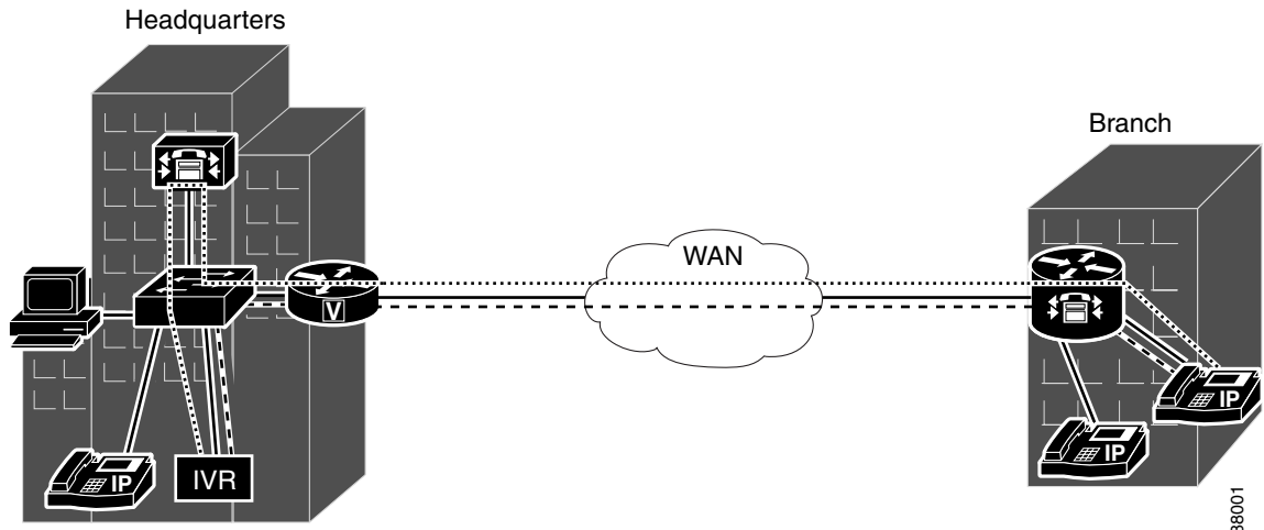
Figure 6 Transcoding Service
