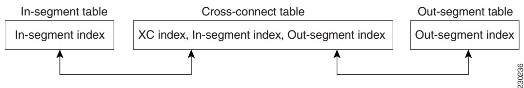
Figure 2 MPLS-LSR-STD-MIB Indexing
