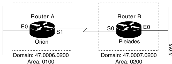
Figure 12 CLNS Interdomain Static Routing
