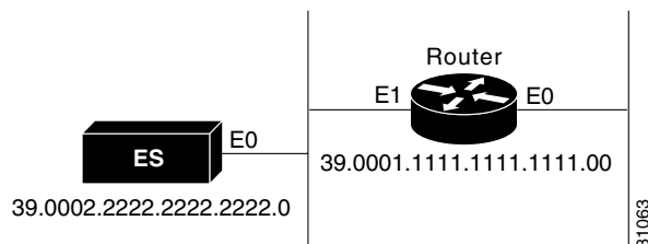
Figure 10 Static Routing
