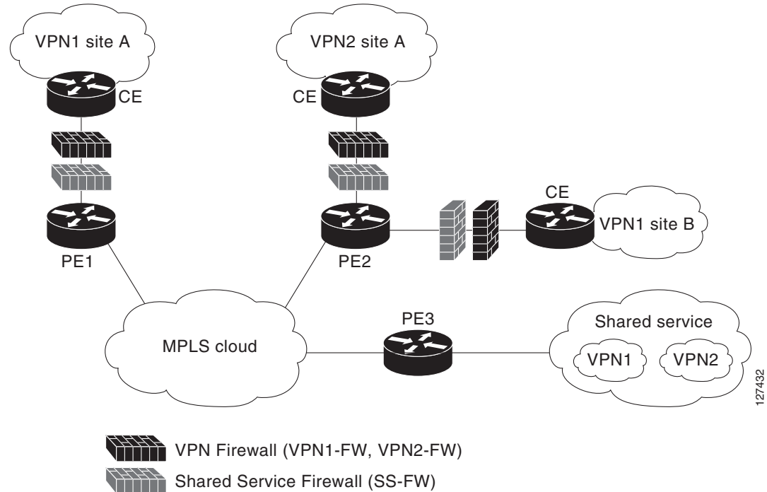
Figure 4 Distributed Network
