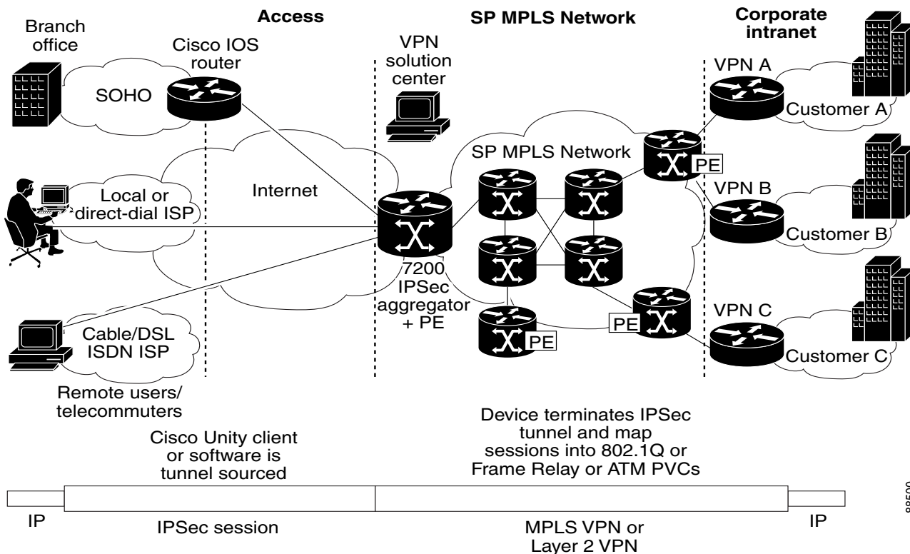
Figure 2 IPsec-to-MPLS and Layer 2 VPNs
