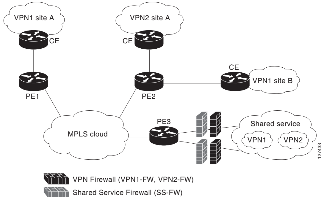
Figure 5 Hub-and-Spoke Network
