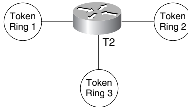
Figure 23 Router with Three Token Rings Configured as a Multiport Bridge
