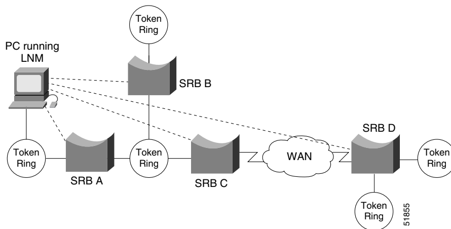
Figure 8 LNM Linking to a Source-Route Bridge on Each Local Ring
