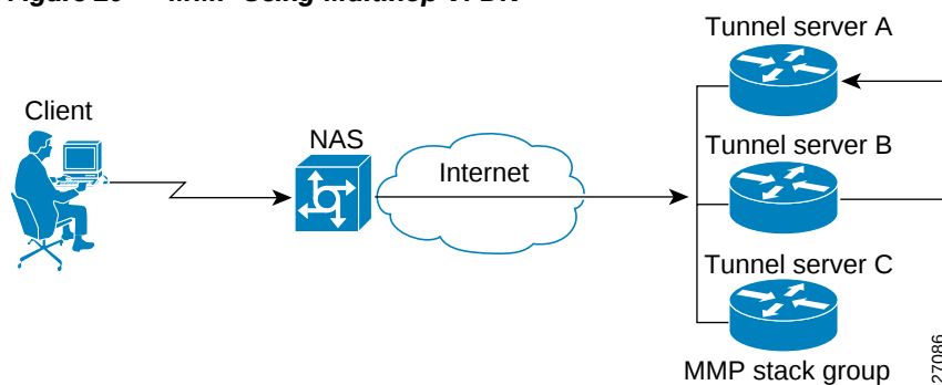
Figure 20 MMP Using Multihop VPDN
