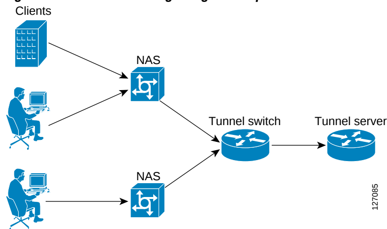
Figure 22 Tunnel Switching Using Multihop VPDN
