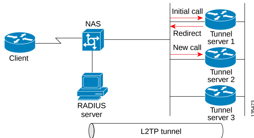
Figure 21 L2TP Redirect Scenario
