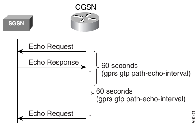
Figure 7 Dynamic GTP Path Echo Interval Request Sequence in Path Success Mode
