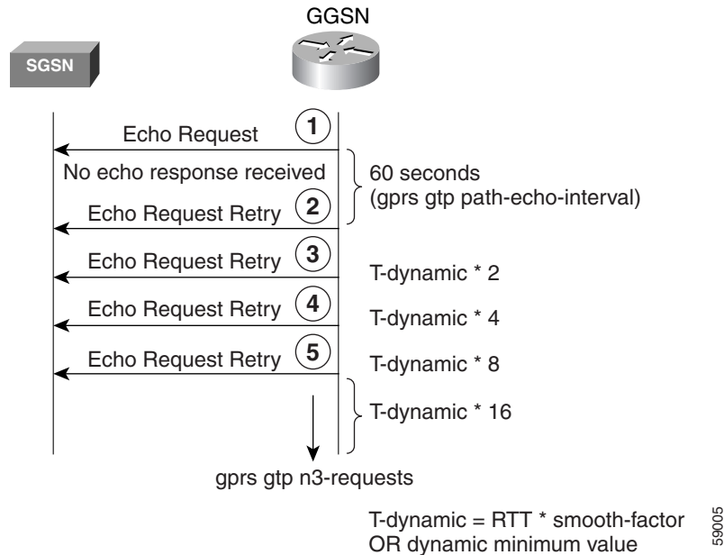
Figure 9 Dynamic Echo Timing Request Sequence in Path Failure Mode
