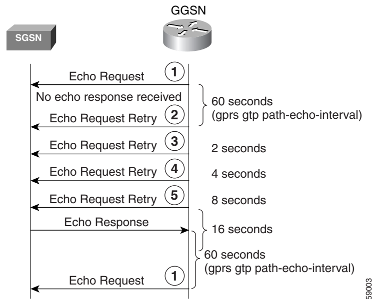
Figure 6 Default Echo Timing with Echo Response Received Within N3 \times T3 Retransmissions
