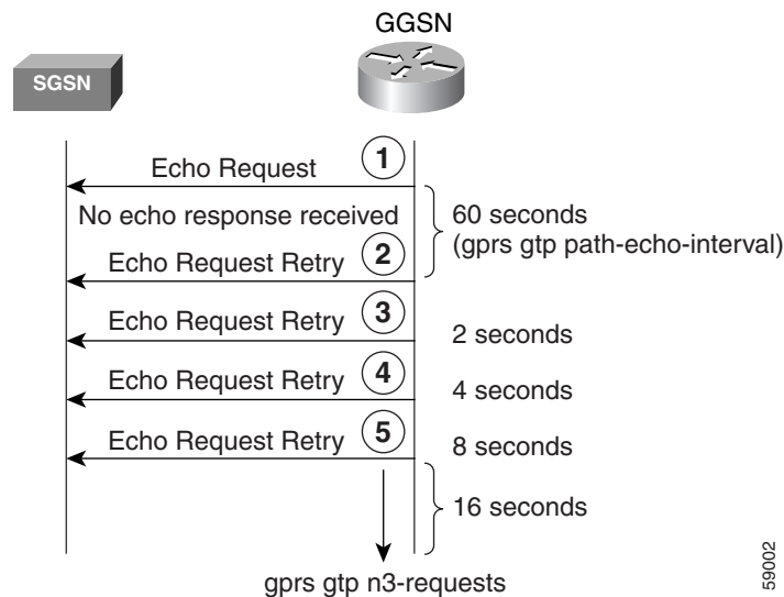
Figure 5 Default Echo Timing Request Sequence in Path Failure Mode
