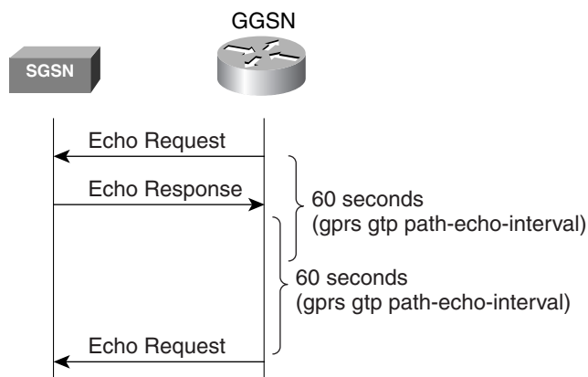
Figure 4 Default GTP Path Echo Interval Request Sequence in Path Success Mode
