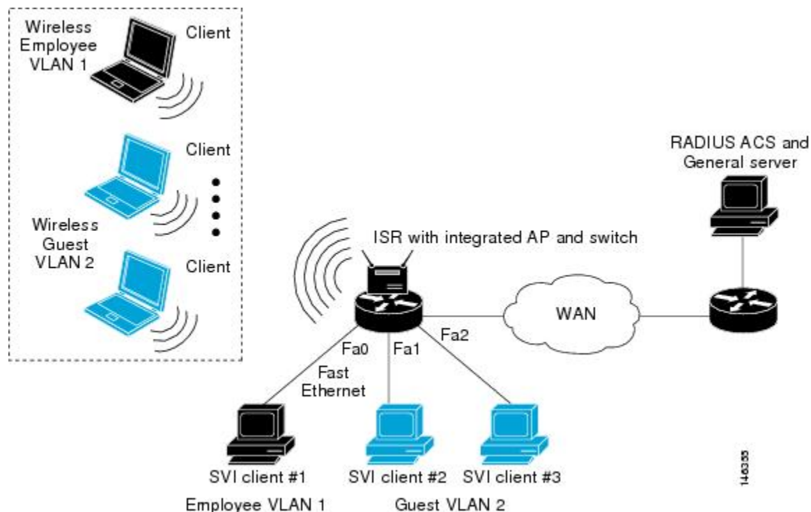
Figure 1 LAN and VLAN Segmentation with Wireless Devices
