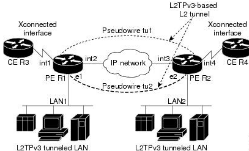
Figure 2: L2TPv3 Operation
