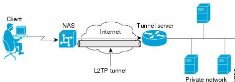
Figure 6: L2TP Architecture
