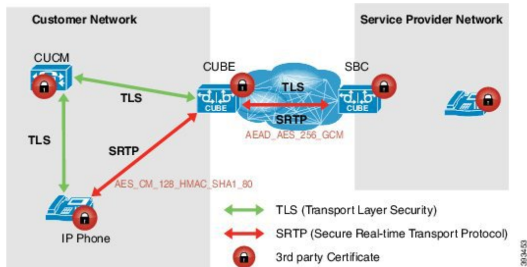
Figure 1: SRTP-SRTP Interworking
