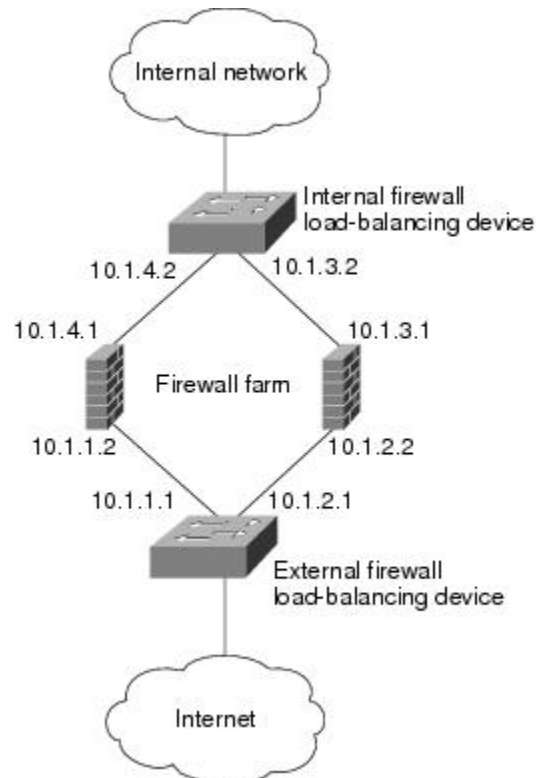
Figure 2: IOS SLB with Layer 3 Firewalls in Different Subnets
