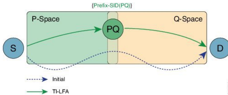
Figure 3: TI-LFA: { Prefix-SID(PQ) }
